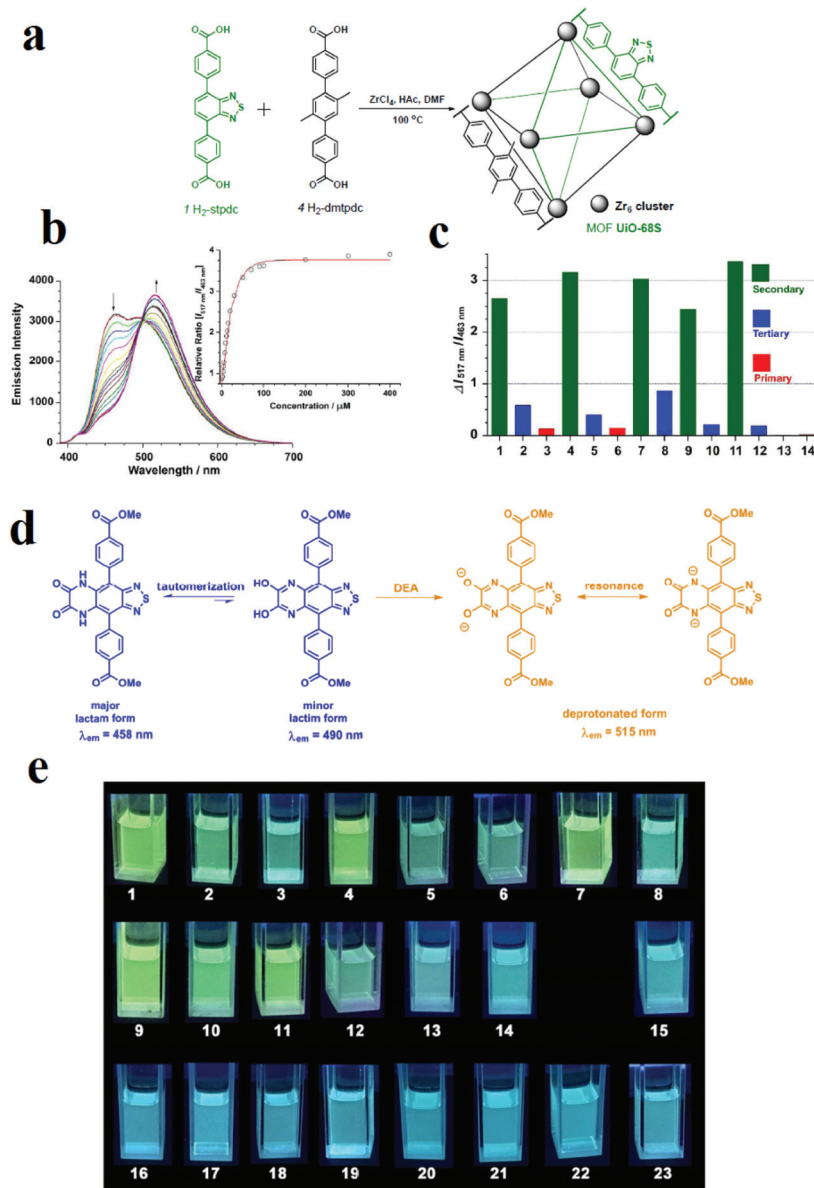
Fig. 24 Application of UiO-68-osdm in amine detection. (a) Synthesis and structure of UiO-68-osdm. (b) Emission spectra of the MOF UiO-68-osdm dispersed in chloroform ( 0.02\text{ mg mL}^{-3} ) upon titration with diethylamine (0 to 0.1\text{ mM} , \lambda_{\text{ex}} = 370\text{ nm} ). Inset: The relative emission ratio ( I_{517\text{ nm}}/I_{463\text{ nm}} ) varies as a function of diethylamine concentration. (c) The changes in the emission ratio of UiO-68-osdm ( \Delta I_{517\text{ nm}}/I_{463\text{ nm}} ) in the presence of different amines ( 0.1\text{ mM} ): 1, diethylamine; 2, triethylamine; 3, propylamine; 4, piperidine; 5, N -methyl piperidine; 6, cyclohexylamine; 7, piperazine; 8, N,N -dimethylpiperazine; 9, diisopropylamine; 10, N,N -diisopropylethylamine; 11, pyrrolidine; 12, N -methyl pyrrolidine; 13, aniline; 14, pyridine. (d) Tautomeric forms of H 2 -ostpdc linker and its typical resonance process and deprotonated form in the presence of diethylamine. (e) Fluorescence photographs of UiO-68-osdm ( 0.2\text{ mg mL}^{-3} ) in chloroform after addition of various amines (#1–14, 0.1\text{ mM} ) and other VOCs (#15–23, 1\text{ mM} ) under a UV lamp ( 365\text{ nm} ). 1: diethylamine; 2: triethylamine; 3: propylamine; 4: piperidine; 5: N -methyl piperidine; 6: cyclohexylamine; 7: piperazine; 8: N,N -dimethylpiperazine; 9: diisopropylamine; 10: N,N -diisopropylethylamine; 11: pyrrolidine; 12: 1-methylpyrrolidine; 13: aniline; 14: pyridine; 15: nitrobenzene; 16: butyraldehyde; 17: methanol; 18: acetone; 19: tetrahydrofuran; 20: acetonitrile; N,N -dimethylformamide; dimethylsulfoxide; 23: benzene. Reproduced with permission from ref. 433.
