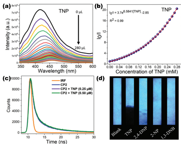
Fig. 6 (a) Fluorescence titration experiment for (26) upon gradual addition of TNP solution in water; (b) Stern–Volmer plot for (26) upon incremental addition of aqueous solution of TNP; (c) lifetime decay profiles of (26) in the presence and absence of TNP solution in water; (d) digital photograph of (26)-coated paper strips after being dipped in aqueous solutions of NACs. Reproduced with permission from ref. 81. Copyright 2018 American Chemical Society.
