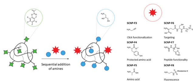
Scheme 2 Overview of SCNP functionalization.
