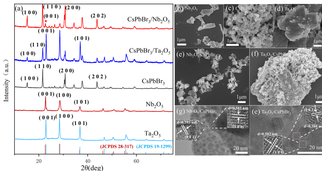
Fig. 6 (a) The XRD patterns for \text{CsPbBr}_3 , \text{Nb}_2\text{O}_5 , \text{Ta}_2\text{O}_5 , and the \text{CsPbBr}_3/\text{Nb}_2\text{O}_5 . The SEM images for (b) \text{Nb}_2\text{O}_5 , (c) \text{CsPbBr}_3 (d) \text{Ta}_2\text{O}_5 , (e) \text{CsPbBr}_3/\text{Nb}_2\text{O}_5 , and (f) \text{CsPbBr}_3/\text{Ta}_2\text{O}_5 . The TEM images (g) for \text{CsPbBr}_3/\text{Nb}_2\text{O}_5 and (h) \text{CsPbBr}_3/\text{Ta}_2\text{O}_5 .
