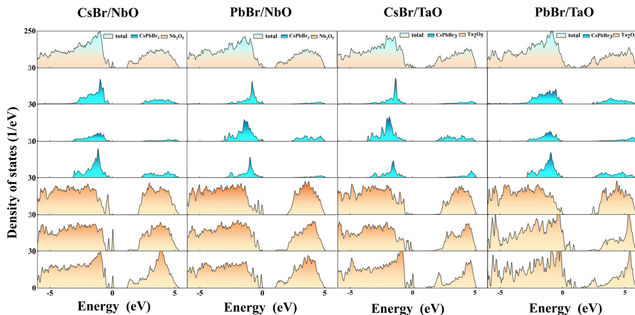
Fig. 3 The calculated DOS plots for the (a) \text{CsBr}/\text{Nb}_2\text{O}_5 , (b) \text{PbBr}/\text{Nb}_2\text{O}_5 , (c) \text{CsBr}/\text{Ta}_2\text{O}_5 , and (d) \text{PbBr}/\text{Ta}_2\text{O}_5 interfacial models.
