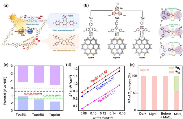
Fig. 5 (a) The mechanism behind photosynthesis of \text{H}_2\text{O}_2 by TTF-BT-COF. 80 (b) Synthesis of TpaBtt, TapbBtt and TaptBtt and directionality of electron transfer between functional motifs and imine linkage in TpaBtt, TapbBtt, and TaptBtt. 82 (c) Energy band values of TpaBtt, TapbBtt, and TaptBtt. 82 (d) Koutecky–Levich plots of TpaBtt, TapbBtt and TaptBtt obtained by RDE measurements. 82 (e) ^{18}\text{O}_2 yields of TpaBtt, TapbBtt and TaptBtt detected by NBT method under light conditions. 82
