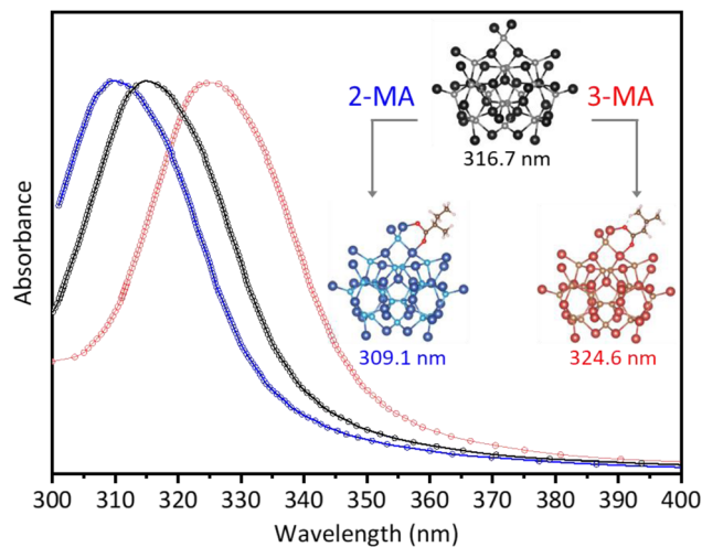
Fig. 3 The computed absorption spectra of pristine Cd 37 S 20 clusters (black trace) with a 2-MA (blue trace) or 3-MA (red trace) molecule coordinated. The corresponding structural models are shown in the inset.
