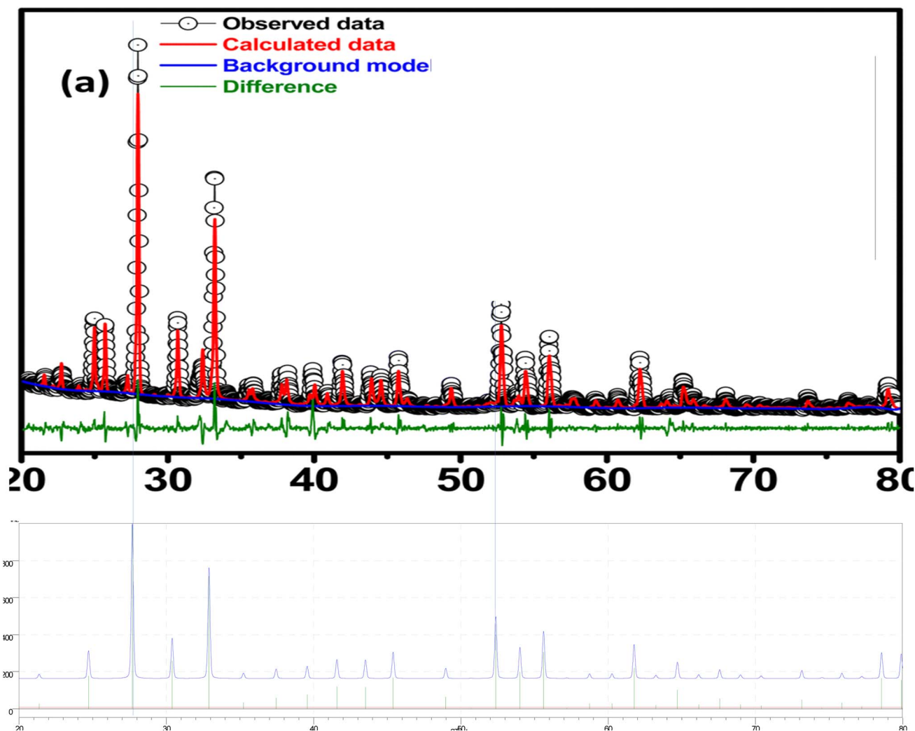
Fig. 1 The comparison of both patterns, experimental (upper diagram) and that of sillenite phase \text{Bi}_{25}\text{FeO}_{40} or \text{Bi}_{24}\text{Mn}_2\text{O}_{40} (bottom pattern, ICSD #41937 and ICSD #75390, respectively; both have nearly the same diffraction pattern). Note that the 2\theta -scale is the same for both patterns.
