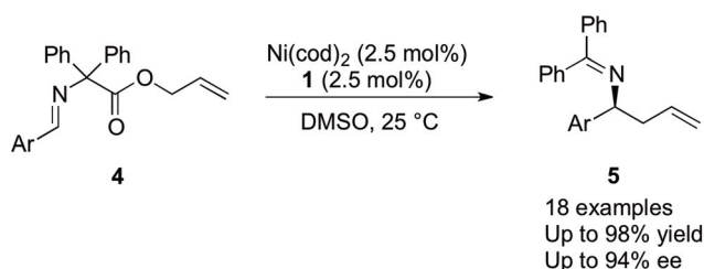
Scheme 2 P,P-1 in Ni-catalysed asymmetric decarboxylative allylic alkylation.
