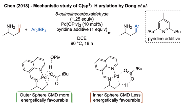
Scheme 31 Mechanistic work elucidating the role of 8-formylquinoline as a transient directing group.
