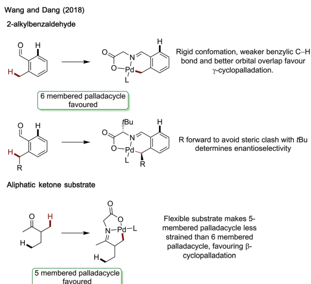
Scheme 30 Origins of regioselectivity with amino acid directing group.
