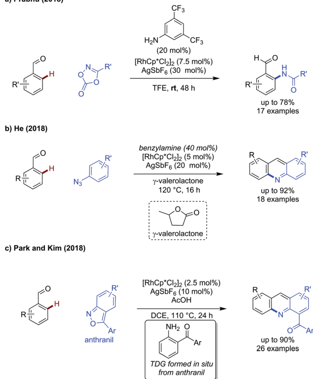
Scheme 3 Rhodium catalysed transient C–N bond forming reactions.
