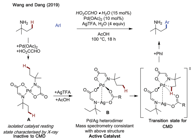
Scheme 32 Mechanistic investigation of the role of silver(I) salts for transient C–H activations.
