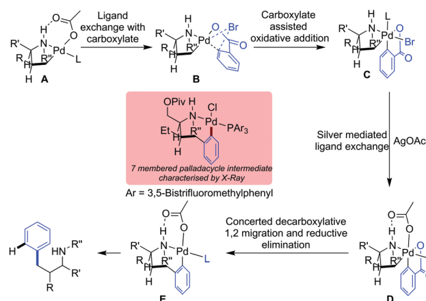
Scheme 26 External directing group free decarboxylative arylation of secondary amines with 2-bromobenzoic acids. Proposed mechanism is shown.
