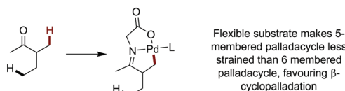
Scheme 30 Origins of regioselectivity with amino acid directing group.
