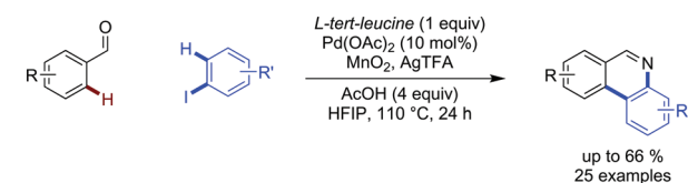
Scheme 7 Palladium catalysed transient C–C bond forming reactions.
