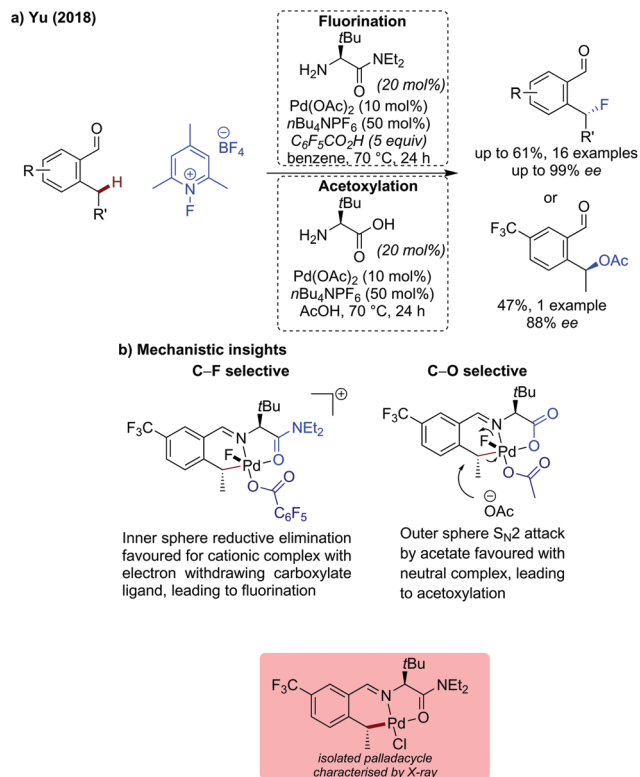
Scheme 14 Palladium catalysed benzylic \text{C}(\text{sp}^3)\text{-H} activation forming C–F and C–O bonds via selective reductive elimination pathways.
