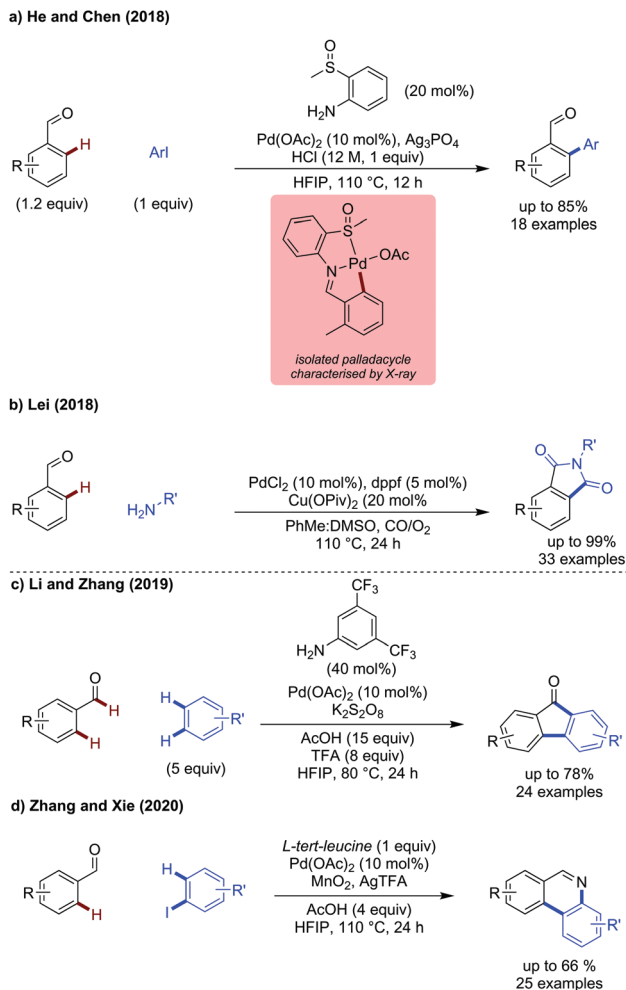
Scheme 7 Palladium catalysed transient C–C bond forming reactions.
