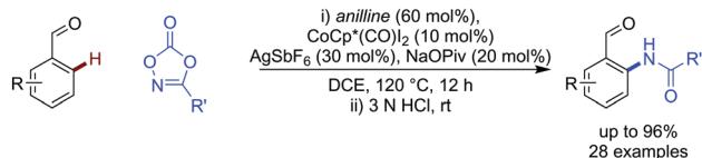
Scheme 6 Cobalt catalysed C–H amination.
