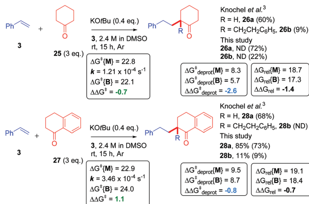
Fig. 13 Application of model to cyclic ketone cakes. ND, not determined. Transition state relative free energies (kcal mol -1 ) for monoadduct ( \Delta G_{rel}(M) ) and bisadduct formation ( \Delta G_{rel}(B) ) for the reaction of cyclic ketones with styrene in DMSO are compared with their previously-reported experimental selectivity. 3 DFT calculations were performed 17–22 with details as in ESI.† Rate constant data was obtained using DMSO- d 6 as solvent, see ESI.† Yields were determined by 1 H NMR by comparison to 1,3,5-trimethoxybenzene (1.0 eq.) as an internal standard. Isolated yields are shown in parenthesis.
