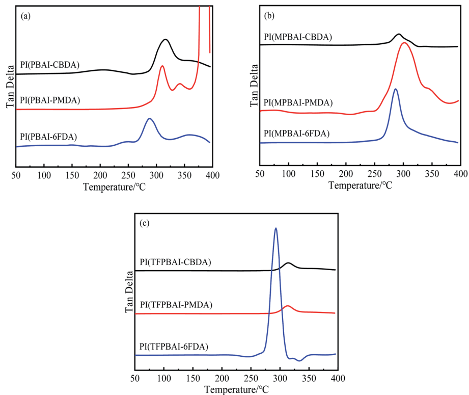
Fig. 3 \tan \delta - T curves of triphenyl imidazole-containing polyimides (a) PIs based on PBAI, (b) PIs based on MPBAI, (c) PIs based on TFPBAI.
