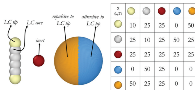
Fig. 1 Molecular models and repulsion parameters implemented for the DPD calculations implemented for the DPD calculations conducted in this study.
