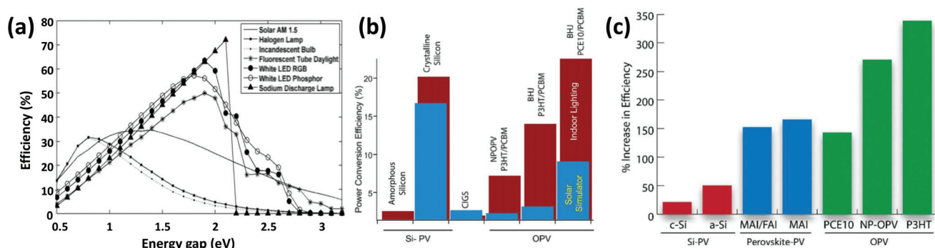
Fig. 2 (a) Energy gap and limiting Shockley–Queisser efficiency of an ideal PV converter with different light sources. Reproduced from ref. 15 and 16 with permission from IEEE Xplore. (b) Comparison of PCE values of silicon and OPV devices under AM 1.5G (blue) and LED (red) light sources. (c) Percent increase in PCE under indoor LED light vs. AM 1.5G simulated solar spectrum. Reproduced from ref. 20 with permission from The Royal Society of Chemistry.
