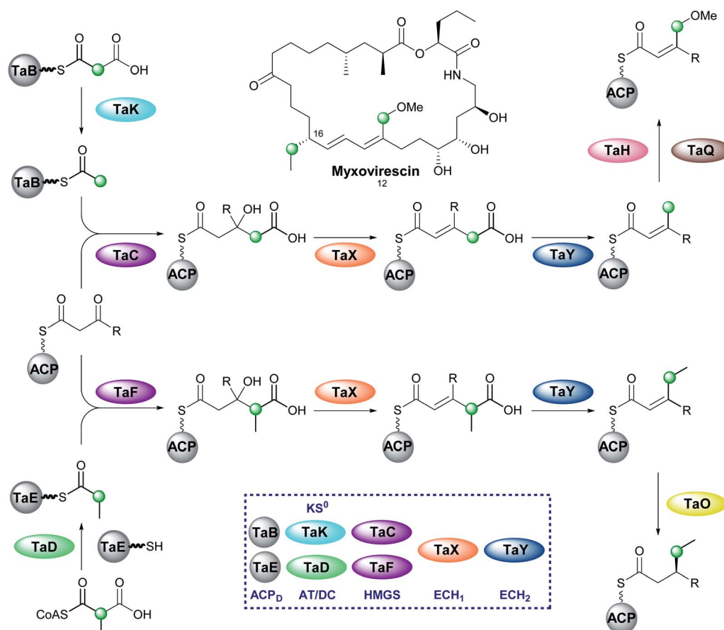
Fig. 25 Incorporation of endo - \beta -methoxymethyl and sat - \beta -ethyl branches in the biosynthesis of myxovirescin. The gene cluster encodes a \text{KS}^0 (TaK) and AT/DC (TaD) to form acetyl-ACP D and propionyl-ACP D respectively. Two ACP/HMGs pairs then select and react either acetyl-ACP D (TaB/TaC) or propionyl-ACP D (TaE/TaF) with the modular \beta -ketothioester. Dehydration and decarboxylation are carried out by the same \text{ECH}_1/\text{ECH}_2 pair (TaX/TaY) prior to oxidation (TaH) and O -methylation (TaQ) to produce the endo - \beta -methoxymethyl at C-12 or reduction (TaO) to produce the sat - \beta -ethyl group at C-16.
