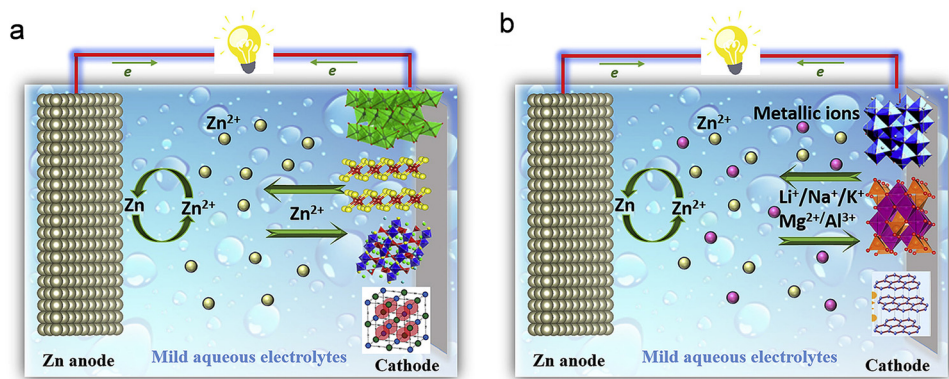
Fig. 7 Comparing the operational principles of Zn-ion batteries. (a) Zn-ion battery ( \text{Zn}^{2+} insertion/extraction mechanism). (b) Hybrid Zn-ion battery ( \text{Li}/\text{Na}/\text{K}/\text{Mg}/\text{Al} insertion/extraction mechanism). Reproduced with permission from ref. 114. Copyright 2019 Elsevier.
