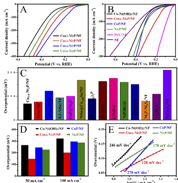
Fig. 4 LSV curves of (A) \text{Co}_{0.6}\text{-Ni}_2\text{P/NF} with different Co contents in a 1 M NaOH solution and (B) \text{Co-Ni(OH)}_2\text{/NF} , \text{CoP/NF} , \text{Ni}_2\text{P/NF} , \text{Co}_{0.6}\text{-Ni}_2\text{P/NF} and \text{Pt/C/NF} . Comparison of the overpotential at current densities of (C) 10 \text{ mA cm}^{-2} and (D) 50 and 100 \text{ mA cm}^{-2} . (E) Tafel plots of \text{Co-Ni(OH)}_2\text{/NF} , \text{CoP/NF} , \text{Ni}_2\text{P/NF} , and \text{Co}_{0.6}\text{-Ni}_2\text{P/NF} .
