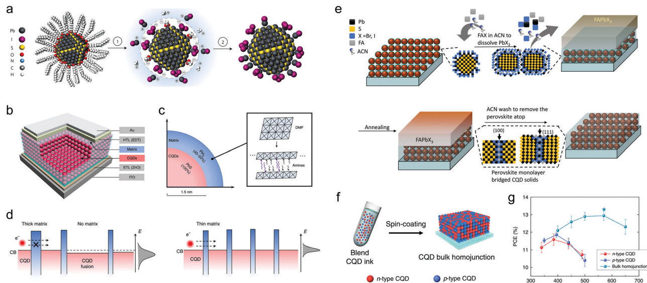
Fig. 3 (a) Solution-phase ligand exchange with metal halide precursors and ammonium acetate. Process 1 (ligand exchange): the bulky oleic acid ligands are replaced by the [\text{PbX}_3]^- anions with the aid of ammonium protons. The CQD surface is stabilized by both [\text{PbX}]^+ and [\text{NH}_4]^+ . Process 2 (CQD precipitation): after ligand exchange, CQDs are precipitated via the addition of toluene, an anti-solvent, and are separated by centrifugation. Reprinted with permission from ref. 17. Copyright 2017, Nature Publishing Group. (b) Schematic diagram of the effective medium model of the CQD absorber in a solar cell, where CQDs (red) assemble in a matrix medium (blue). (c) The matrix consists of \text{PbI}_2 , which is enough to account for the formation of full monolayer coverage on the surfaces of PbS CQDs (bandgap \sim 1.3 eV and diameter \sim 3 nm). The dimensional structure of the matrix can be tuned using solvents. (d) The schematic diagram for the effect of homogeneity of the matrix on the structural and energetic order of CQD film. Confining the matrix dimensionality between the CQDs and improving its homogeneity throughout the film can increase the photocarrier diffusion length and reduces the V_{\text{oc}} deficit. Reprinted with permission from ref. 43. Copyright 2018, Nature Publishing Group. (e) Schematic of the formation of monolayer perovskite bridges among the QDs. The perovskite matrix is formed first by soaking the pre-exchanged CQD films in a FAX ( X = \text{Br}, \text{I} ) solution, where the FAX solution dissolves the \text{PbX}_3^- ligands and perovskite grows between adjacent PbS CQDs. The films are annealed and then washed with acetonitrile to remove excess perovskite. Reprinted with permission from ref. 18. Copyright 2014, Elsevier. (f) The bulk-homojunction films were fabricated by depositing the blended CQD inks comprising n-type and p-type CQDs. (g) Thickness-dependent PCE for bulk-homojunction devices and n-type CQD devices. Bulk-homojunction devices enable the use of much thicker CQD films compared with the case of n-type CQD devices, indicating the increase of carrier diffusion length. Reprinted with permission from ref. 49. Copyright 2020, Nature Publishing Group.
