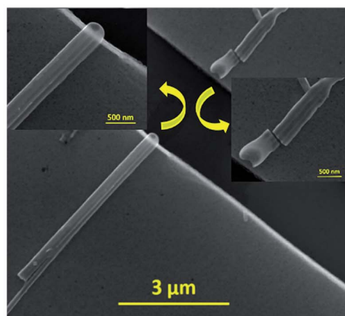
Fig. 9 (a) In the 'Model C' breakdown, the J - V curve displays mixed features of nonlinearity along with sudden big steps in J before the breakdown point which may be the characteristics for breaking of the bridge between the nanotubes in the bundle. SEM images exhibit a bundle of 3 EGTNT (b) before and (c) after the breakdown; magnified SEM images are also displayed in the insets.
