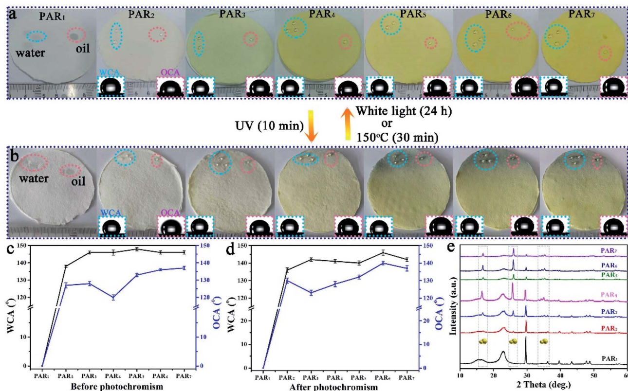
Fig. 4 (a) Optical pictures of PAR i before photochromism; (b) optical pictures of PAR i after photochromism. The illustrations correspond to the contact angle pictures of water and oil. The blue dashed circles are water and the red dashed circles are rapeseed oil. The statistics of the WCA and OCA of PAR i before photochromism (c) and after photochromism (d). (e) XRD patterns of PAR i .
