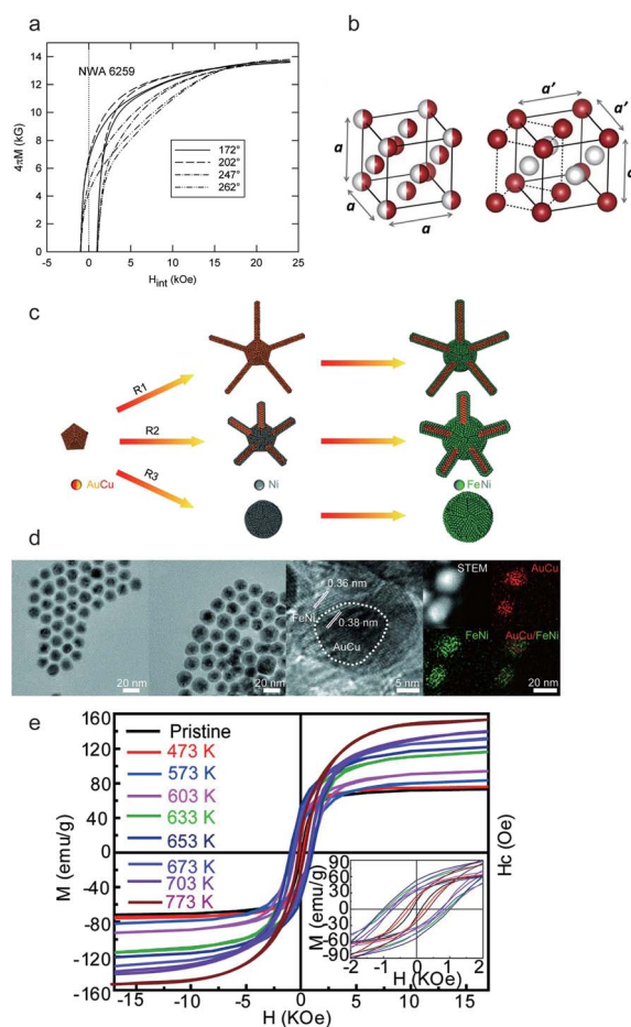
Fig. 7 (a) Magnetic hysteresis of NWA 6259 tetraenaite; (b) representations of the cubic (A1) and tetragonal (L1 0 ) unit cells of FeNi; (c) schematic images of the synthesis procedure of AuCu/FeNi (core/shell) nanocrystals; (d) TEM images of AuCu/FeNi (core/shell) nanostructures at different shell thicknesses. (e) The magnetic hysteresis loops of AuCu/FeNi (core/shell) nanocrystals with the stoichiometry of Fe 46 Ni 54 at different annealing temperatures, and the inset images show the corresponding magnified hysteresis loops. Reproduced from ref. 84, 85 and 87 with the permission of AIP Publishing, Elsevier, and American Chemical Society.
