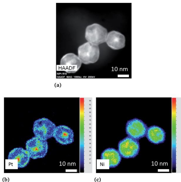
Fig. 1 \text{Ni}_3\text{Pt} colloidal synthesis performed at 225 °C. (a) STEM-HAADF image and chemical mappings using EDX mode with the concentration scale demonstrate that (b) Pt ( L_{\alpha} line) is predominantly located in the core and (c) Ni ( K_{\alpha} line) mainly in the shell.
