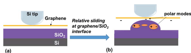
Fig. 10 Interaction with polar modes at the interface of graphene and the SiO 2 substrate before (a) and after (b) the relative sliding occurring at the interface.
