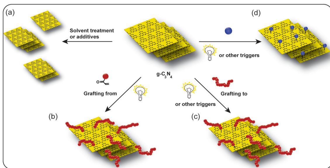
Scheme 3 Approaches towards improvement of g\text{-C}_3\text{N}_4 dispersibility: (a) utilization of solvent mixtures (e.g. water/ethylene glycol (EG)), (b) grafting polymers from g\text{-C}_3\text{N}_4 via free radical polymerization, (c) grafting polymers to g\text{-C}_3\text{N}_4 via double bond containing preformed polymers and (d) photofunctionalization with ene containing small molecules.
