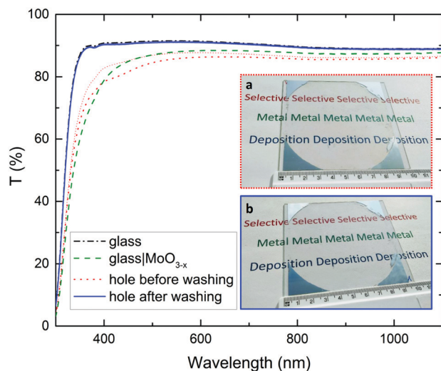
Fig. 3 Characterization of a 10 cm diameter hole in a silver film. Transmittance spectra (referenced to air) of a 10 cm diameter hole in a 50 nm thick silver film fabricated by printing an FTS layer using a PDMS stamp on \text{MoO}_{3-x} (15 nm)/glass substrate. The thin and thick dashed red lines are respectively the highest and average transparency of that measured at seven different locations in the aperture. (a) Sample after metal evaporation. (b) Sample after washing with tetrabutylammonium fluoride/tetrahydrofuran solution and water.
