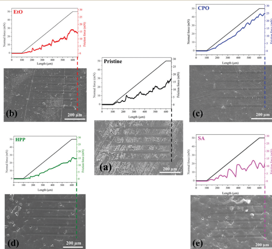
Fig. 6 Friction and plastic deformation behaviors for different treated samples where pristine is (a), EtO (b), CPO (c), HPP (d) and SA (e).
