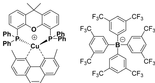
Fig. 1 Chemical structure of complex 1 with counterion \text{tfpb}^- . Structure of complex 1 obtained by single crystal X-ray crystallography, which is fully consistent with that published previously, is given in the ESI† Fig. S8. CCDC 2012235.
