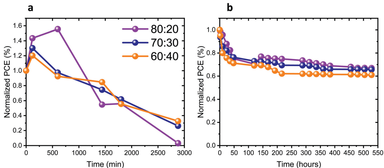
Fig. 7 (a) Stability under 1 sun illumination of complete solar cells with different ratios of Pb : Sn as discussed in this work. (b) Stability of the cells stored under an inert atmosphere and measured in the open air with encapsulation.
