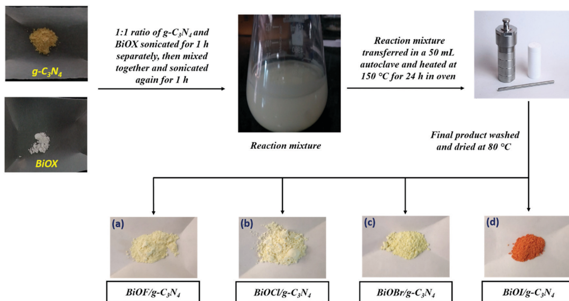
Scheme 2 Schematic representation of the hydrothermal synthesis of BiOX/ g\text{-}C_3N_4 composites (a) BiOF/ g\text{-}C_3N_4 , (b) BiOCl/ g\text{-}C_3N_4 , (c) BiOBr/ g\text{-}C_3N_4 and (d) BiOI/ g\text{-}C_3N_4 .
