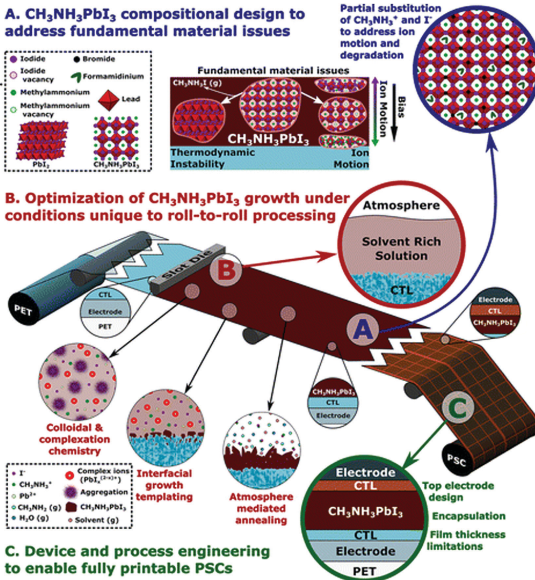
Fig. 9 Summary of research directions necessary to fuel PSC technological translation by slot-die R2R coating. (A) Material engineering can address intrinsic ion diffusivity and degradation of CH 3 NH 3 PbI 3 , (B) optimization of perovskite growth under R2R conditions is necessary to reach performance requirements, and (C) device engineering is required to extend the device life and expand the material toolbox for the PSC design. Reproduced with permission from ref. 116. Copyright © 2016 American Chemical Society.
