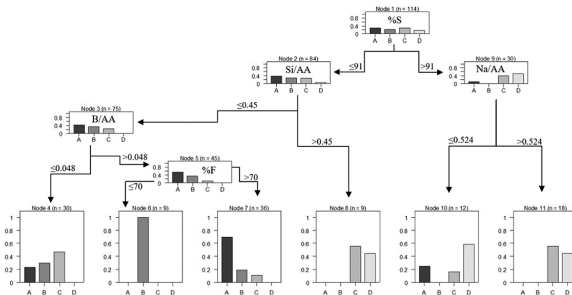
Fig. 3 DT flowchart of the ctree function.
