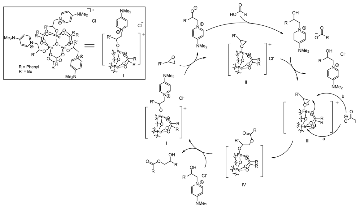
Scheme 3 Proposed catalytic cycle for the FeCl 3 /DMAP catalyzed nucleophilic ring opening reaction of epoxides with carboxylic acids.
