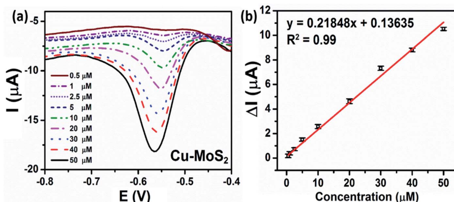
Fig. 9 (a) DPV curves of Cu-MoS 2 -75/SPE in 0.1 M PBS (pH 5) containing CAP (0.5–50 \mu M) at a scan rate of 6 mV s -1 corresponding to the calibration plots of the peak current vs. various concentrations of CAP (b) along with error bars.
