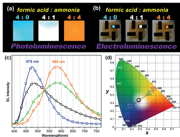
Fig. 7 (a) Photographs of thin film emission dependent on pH under a UV lamp and (b) the image of LED devices under operation. (c) EL spectra and (d) CIE chromaticity diagram dependent on formic acid to ammonia ratio (□) 4 : 0, (○) 4 : 1, (△) 4 : 2, and (▽) 4 : 4.
