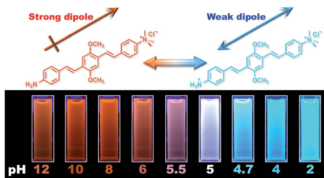
Fig. 1 (Top) Diagram of the protonation of ATAOPV : on the left is the non-protonated molecule whose chemical formula is abbreviated as NH_2\text{-OPV-NMe}_3^+ , on the right is the protonated molecule NH_3^+\text{-OPV-NMe}_3^+ . (Bottom) Photographs of ATAOPV multicolor emission as a function of pH 12–2 in solution ( 10^{-5} M in H_2O ).
