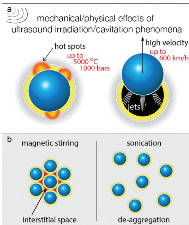
Fig. 6 The main mechanical/physical effects derived from ultrasound irradiation due to the cavitation phenomena (a) and the difference in the extend of de-aggregation (b).
