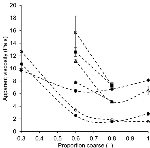
Fig. 3 Impact of PSD on apparent viscosity. If no data points are given, the viscosity of samples was too high to be measured. Quartz beads model systems with 28% fat ( \diamond ) and model chocolate samples with 28 ( \square ), 30 ( \triangle ) and 36% fat ( \circ ). All samples are without lecithin. Open symbols: size ratio 1:4; closed symbols: size ratio 1:6. Dashed lines were added to guide the eye.
