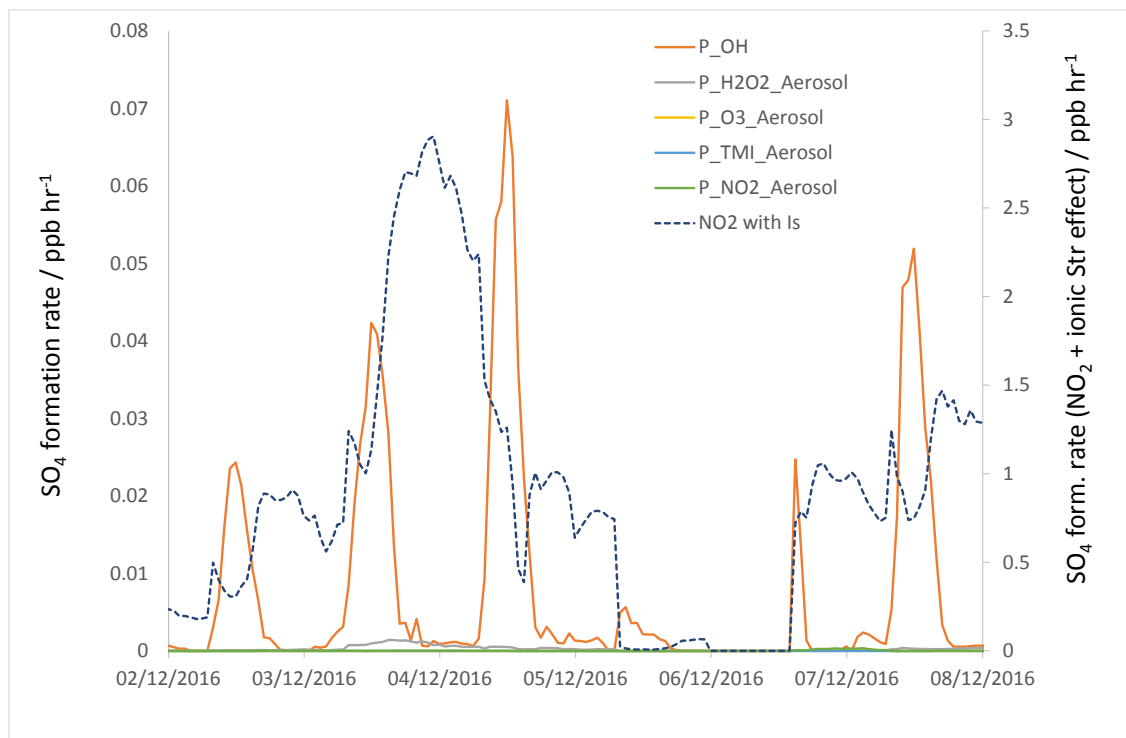
Figure 6: Modelled \text{SO}_4 formation rates (converted to \text{ppb hr}^{-1} ) through reaction of \text{SO}_2 with OH (orange line), condensed phase reactions (all case B) with \text{H}_2\text{O}_2 (grey), \text{O}_3 (yellow), transition metals (blue) and \text{NO}_2 (green). Dashed line, second y axis: \text{NO}_2 reaction considering impacts of ionic strength on \text{NO}_2 + \text{S(IV)} reaction kinetics (i.e. case C). See Fig S5 (Supp Info) for expansion of the \text{H}_2\text{O}_2 , \text{O}_3 and TMI timeseries.
