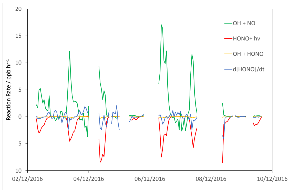
Figure 3: Timeseries of the observationally-derived components of in-situ HONO formation and destruction: reactions of OH + NO (R2), OH + HONO (R3), HONO + hv (R4), plus the observed rate of change of HONO, d[HONO]/dt.
