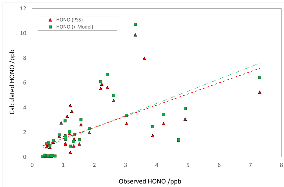
Figure 5: Correlation between observed HONO and PSS-predicted mixing ratios (red triangles), regression line (red dashes), and model calculated HONO levels (see text; green squares) and associated regression (green dots).
