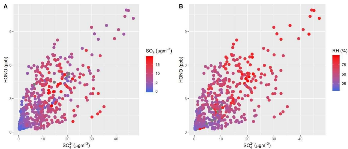
Figure 2 – Relationship between HONO and \text{SO}_4 concentrations, coloured by \text{SO}_2 abundance (panel A) and by relative humidity (RH, panel B), during the 2 – 10 Dec focus period. The data show a limited impact of \text{SO}_2 , but the highest levels of both HONO and \text{SO}_4 are associated with elevated humidity.
