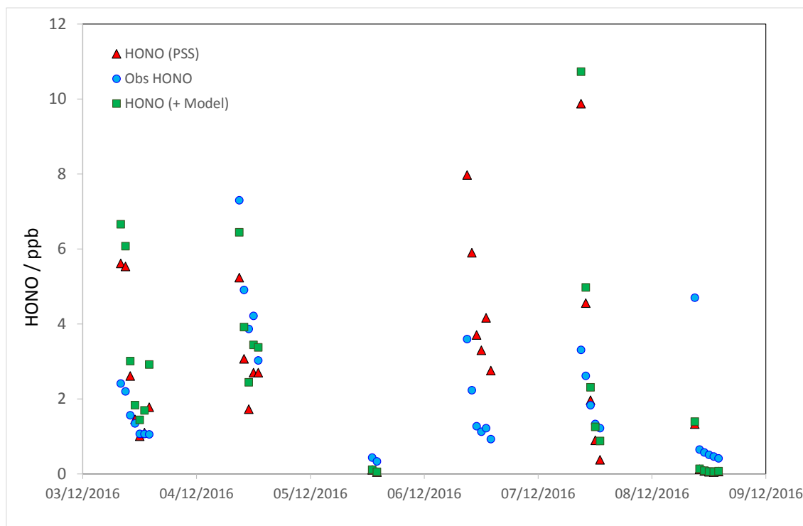
Figure 4: Timeseries of observed daytime HONO mixing ratios (blue circles), steady state calculated HONO mixing ratios - HONO PSS, as derived from application of Equation E1 - (red triangles) and model calculated HONO (see text; green squares)
