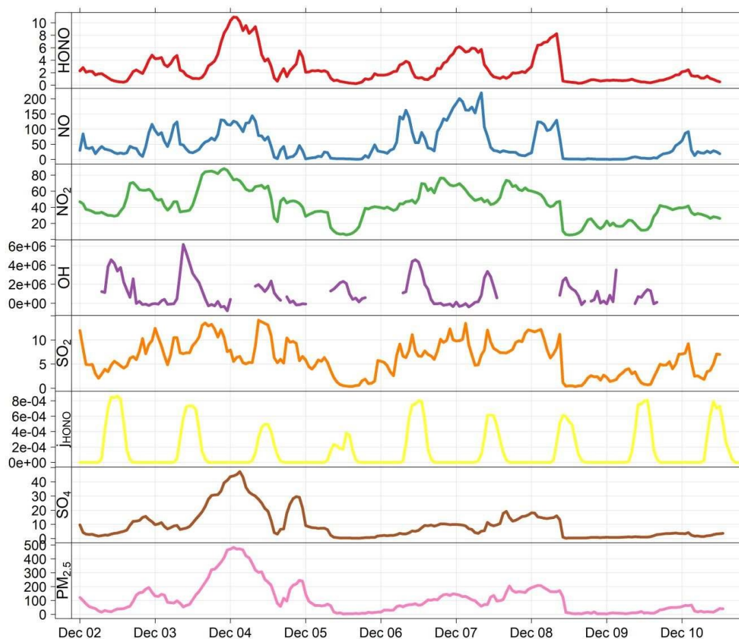
Figure 1: Measured timeseries for HONO (ppb), NO (ppb), NO 2 (ppb), OH (molec cm -3 ), SO 2 (ppb), j_{\text{HONO}} (s -1 ), SO 4 (AMS; μg m -3 ) and PM 2.5 (TEOM FDMS; μg m -3 ) at the IAP tower site during the APHH Beijing winter campaign, 2016
