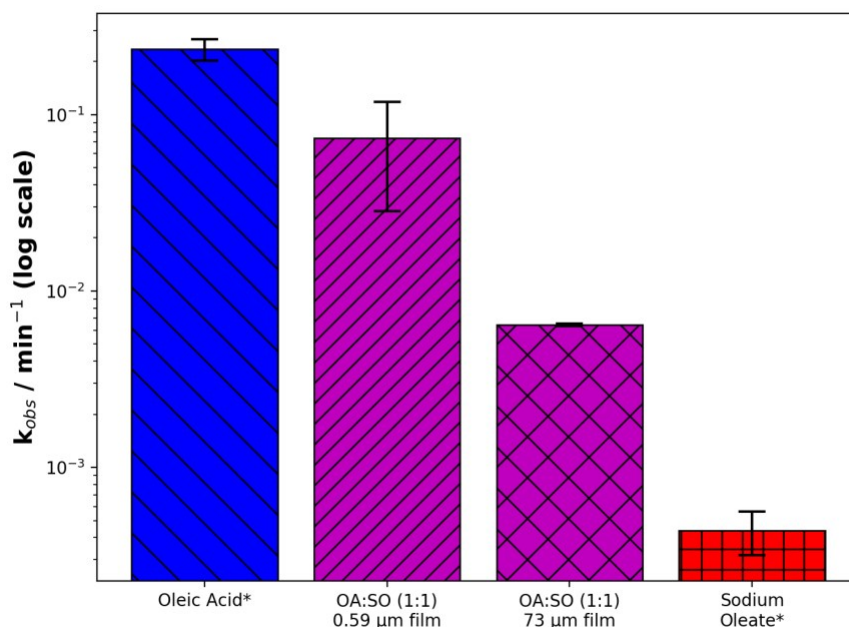
Figure 4. Comparison of k_{obs} between a capillary coating of oleic acid (liquid), two coatings of self-assembled oleic acid-sodium oleate proxy (semi-solid: 0.59 & 73 \mu\text{m} thick) and a coating of sodium oleate (solid). *The oleic acid and sodium oleate decays were followed by Raman microscopy, using the C=C band at 1650 \text{cm}^{-1} . The thickness of the oleic acid and sodium oleate coatings was measured to be \sim 50 \mu\text{m} based on the X-ray attenuation of these samples compared to self-assembled coatings of known thickness. (OA: oleic acid; SO: sodium oleate). [\text{O}_3] = 77 \pm 5 \text{ ppm} .
