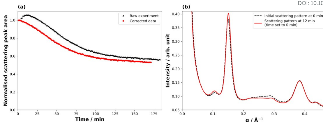
Figure 2. Illustration of data correction (film thickness: 73 \pm 2 \mu\text{m} ). (a) Scattering peak area vs time exposed to ozone, both raw and corrected data plotted. (b) SAXS patterns of the sample at the beginning of the experiment (black dashed line) and at the time (after 12 min) at which the peak scattering area was measured, which was defined as t = 0 for the decay of the lamellar phase (red solid line).
