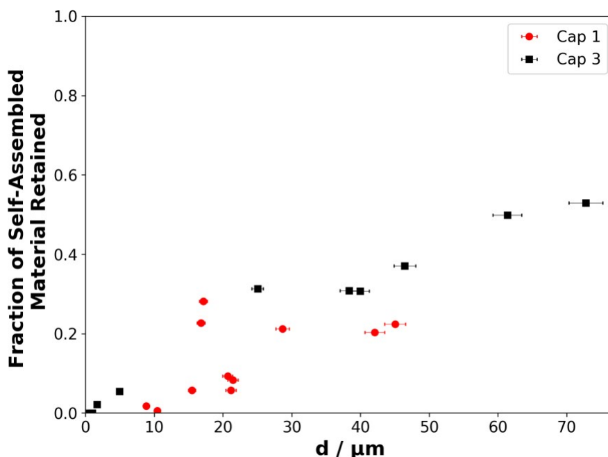
Figure 5. The fraction of self-assembled material retained at the end of each experiment (after \sim 175 min of ozonolysis), when the reaction was deemed to have stopped or slowed significantly, as a function of film thickness. Symbols, colours and labels correspond to the same experiments presented in Fig. 3.
