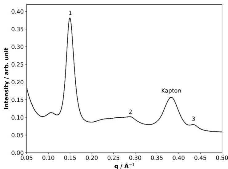
Figure 1. The initial SAXS pattern of a 73 \pm 2 \mu\text{m} thick film. Numbers indicate the lamellar phase Bragg peaks. The scattering peak from Kapton film on the X-ray detector is also labelled and was used as an internal standard.
