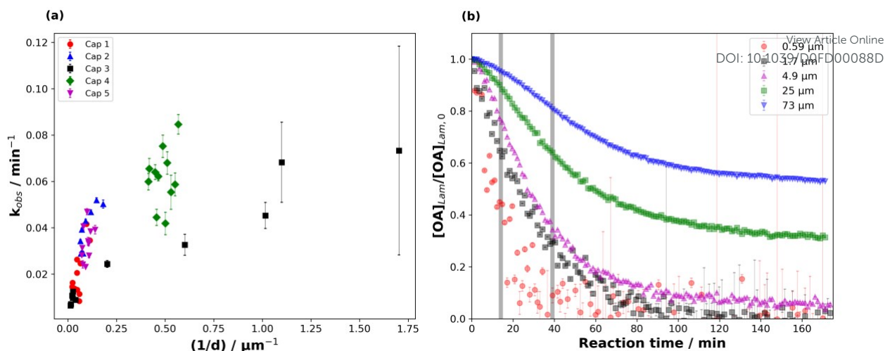
Figure 3. The observed pseudo-first order decay constant ( k_{\text{obs}} ) as a function of (a) inverse film thickness ( 1/d ), demonstrating the film-thickness dependence of the reaction kinetics. Different capillary (“Cap”) experiments are distinguished by different colours and symbols. (b) Decay plots of the normalised amount of lamellar oleic acid ( [\text{OA}]_{\text{Lam}}/[\text{OA}]_{\text{Lam},0} ) vs reaction time ( t ) at different thicknesses – data are from one capillary experiment (“Cap 3”) and grey bars indicate the reaction times between which k_{\text{obs}} was measured for films with d > 2.5 \mu\text{m} . [\text{O}_3] is 77 \pm 5 \text{ ppm} .
