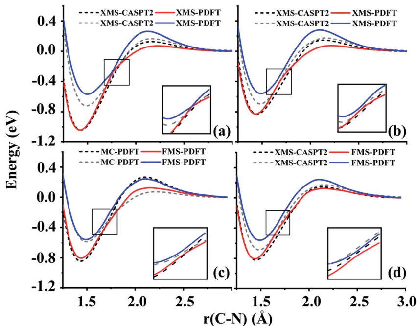
Fig. 3 (a) and (b) Comparison of XMS-PDFT with XMS-CASPT2 for the two lowest potential energy curves along the CN bond dissociation of HNCN with the \tau(\text{HNCN}) torsion angle at 175° and 150° respectively. (c) and (d) Comparison of FMS-PDFT with MC-PDFT and XMS-CASPT2 for the two lowest potential energy curves along the CN bond dissociation with the \tau(\text{HNCN}) torsion angle at 150°. The curves from 2.0 to 2.5 Å are calculated with numerically optimized VMS-PDFT instead of FMS-PDFT.
