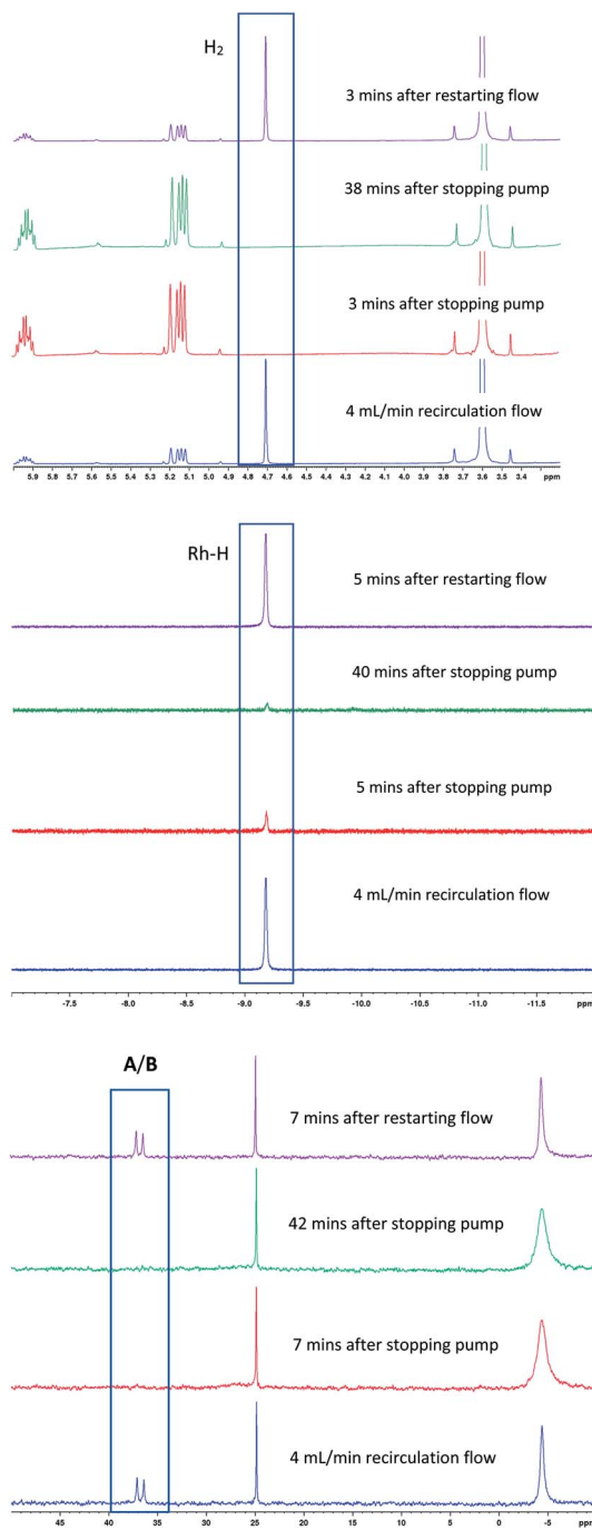
Fig. 13 ^1\text{H} and ^{31}\text{P}\{^1\text{H}\} FlowNMR spectra of [\text{Rh}(\text{CO})_2(\text{acac})] + 6\text{PPh}_3 catalysed hydroformylation of 1-hexene in toluene at 50 °C and 12 bar of \text{H}_2/\text{CO} (1 : 1) during stop/start cycling of flow. [\text{Rh}(\text{CO})_2(\text{acac})] = 2.5 \text{ mM} , [1\text{-hexene}] = 500 \text{ mM} , [\text{PPh}_3] = 15 \text{ mM} .
