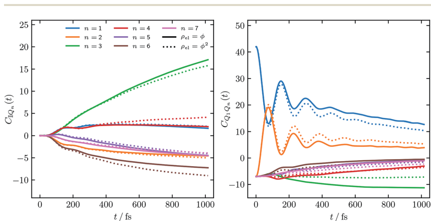
Fig. 1 Constituent correlation functions of the FMO population, with T = 77 K, and \tau_c = 50 fs and an initial excitation of site |1). The solid and dotted lines correspond to the electronic initial conditions having been sampled either from \phi(X,P) or \phi^2(X,P) . In eqn (15) this corresponds to a = 1 and a = 2 respectively.
