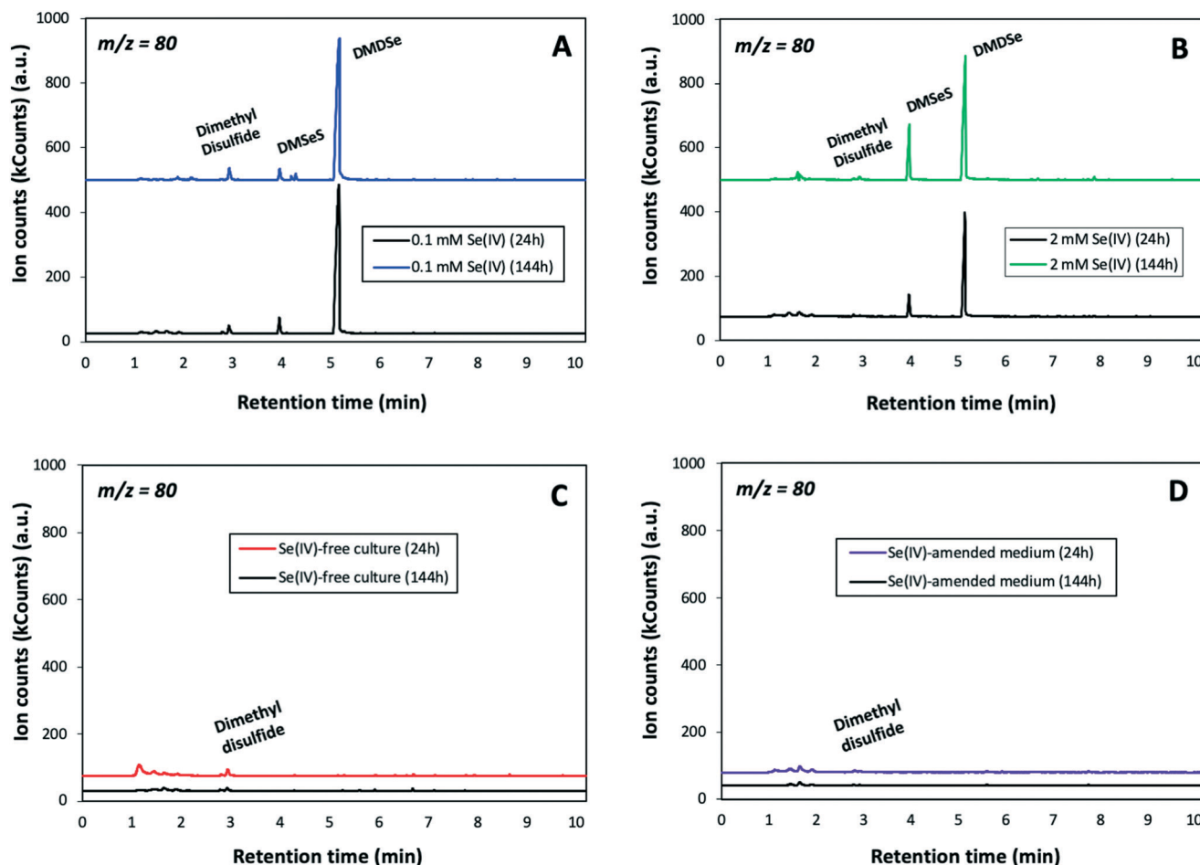
Fig. 9 GC-MS chromatograms of the headspace gas of S. bentonitica cultures supplemented with \text{Se}^{\text{IV}} (0.1 and 2 mM) (A and B) and without \text{Se}^{\text{IV}} (C), after 24 and 144 h of incubation. \text{Se}^{\text{IV}} -amended medium (2 mM) chromatograms after 24 and 144 h of incubation were used as control (D). All GC-MS chromatograms were obtained by selecting the 80 m/z ion specific for selenium.
