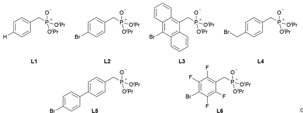
Chart 2 Overview of the phosphonate ester ligands L1 – L6 used within this work.
