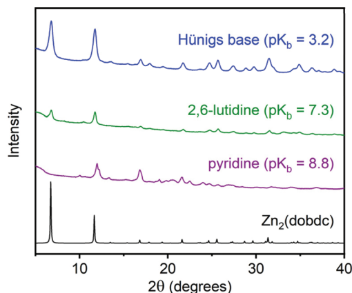
Fig. 7 Powder X-ray diffraction patterns ( \lambda = 1.5406 \text{ \AA} ) of Zn_2(dobdc) prepared under mechanochemical conditions with different organic bases. The simulated pattern based on the previously reported single-crystal X-ray diffraction structure of Zn_2(dobdc) is included for reference. 55
