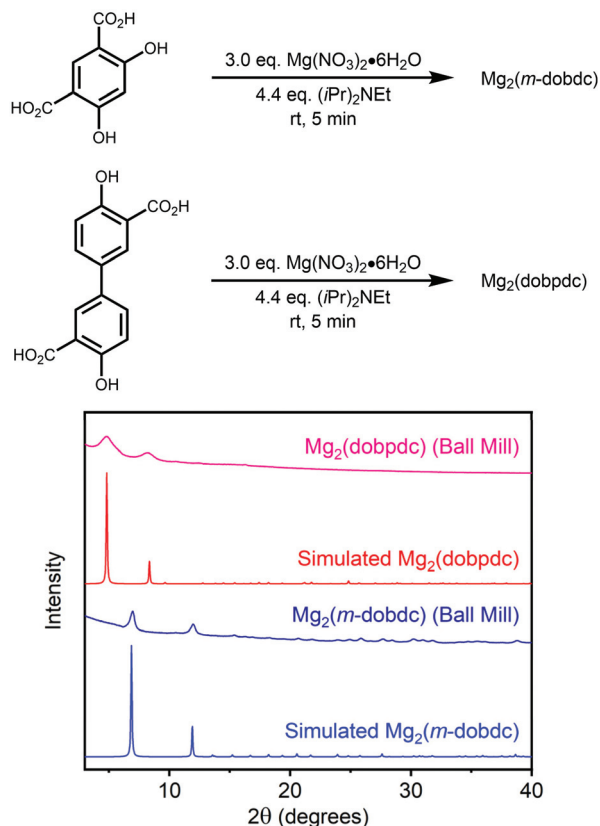
Fig. 6 Powder X-ray diffraction patterns ( \lambda = 1.5406 \text{ \AA} ) of Mg_2(m-dobdc) (blue) and Mg_2(dobpdc) (red) prepared under mechanochemical conditions. The simulated patterns based on the previously reported single-crystal X-ray diffraction structures of the isostructural frameworks Co_2(m-dobdc)^{54} and Zn_2(dobpdc)^{56} are included for reference.
