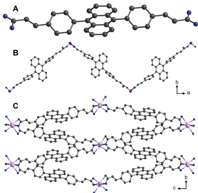
Fig. 1 Solid-state structures of (A) H 2 L, (B) one-dimensional coordination polymer [Zn(L)(DMF)_2]_n (1) and (C) a three-dimensional metal-organic framework [Cd(L)(DMF)] \cdot DMF_n (2) based on 4,4'-(9,10-anthracenediyl)dicinnamic acid (H 2 L). Solvent molecules and hydrogen atoms were omitted for clarity. Colour code: C, black; O, blue; Zn, purple; Cd, pink.
