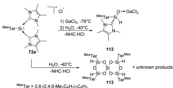
Scheme 43 Activation of H 2 O by the silyliumylidene-NHC complex 72a .
