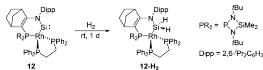
Scheme 8 Activation of H 2 by the cyclic (imino)metal substituted silylene 12 .
