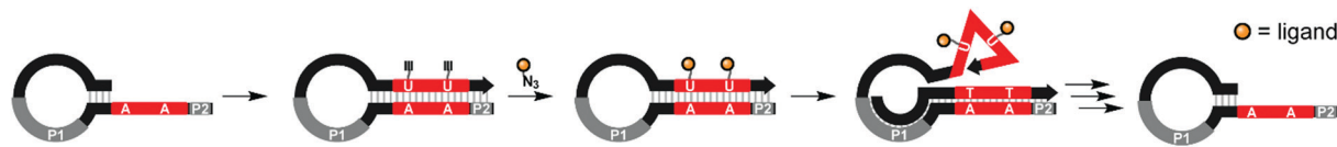
Fig. 5 SELMA (selection of modified aptamers) process: a library of hairpins is extended by polymerase which incorporates alkyne-modified uridines. Azide-modified ligands are conjugated through Cu-mediated click chemistry. Extension from primer site P1 ejects the ligand-decorated strand from the hairpin, allowing it to fold into a three-dimensional shape, which is screened against a target compound. Through multiple subsequent steps the starting hairpin can be regenerated for further selection rounds (ref. 21).
