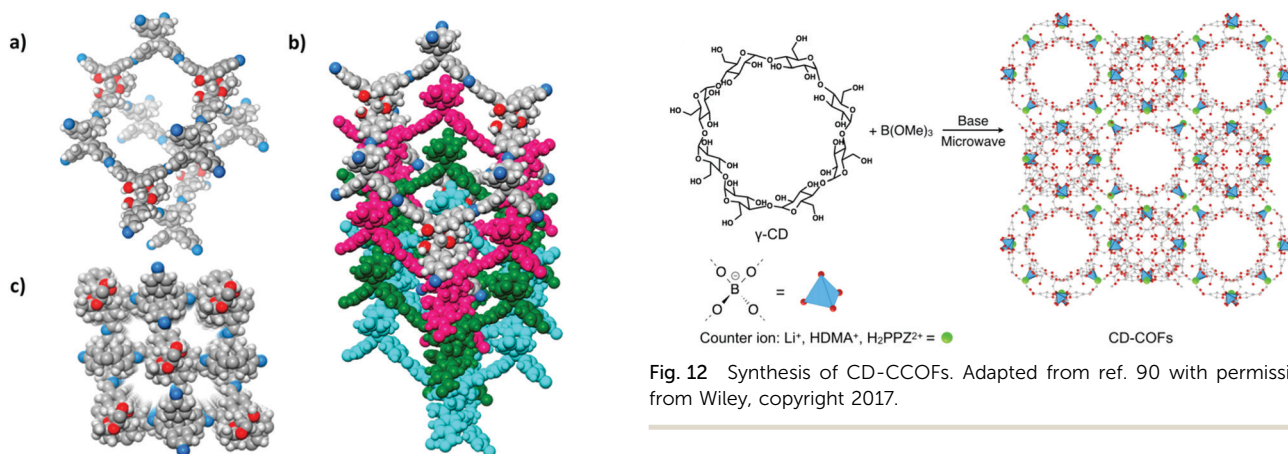
Fig. 11 Structural representation of CCOF 5. (a) Adamantine-like cage in the diamond net. (b) Structure viewed along the a -axis showing 4-fold interpenetration of a diamond net. (c) Two kinds of 1D channels long the c -axis. C gray; N blue; H white; O red. Adapted from ref. 86 with permission from the American Chemical Society, copyright 2018.
