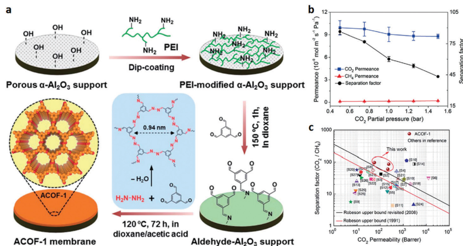
Fig. 15 (a) Schematic illustration of synthesizing the ACOF-1 membrane on the porous \alpha - \text{Al}_2\text{O}_3 support. (b) CO 2 permeance and CO 2 /CH 4 separation factor of the ACOF-1 membrane as a function of the CO 2 partial pressure at 120^\circ\text{C} . (c) Permeability vs. separation factor of various membranes and the upper bound correlation for CO 2 /CH 4 separation. Reproduced with permission from ref. 124. Copyright 2018, Royal Society of Chemistry.
