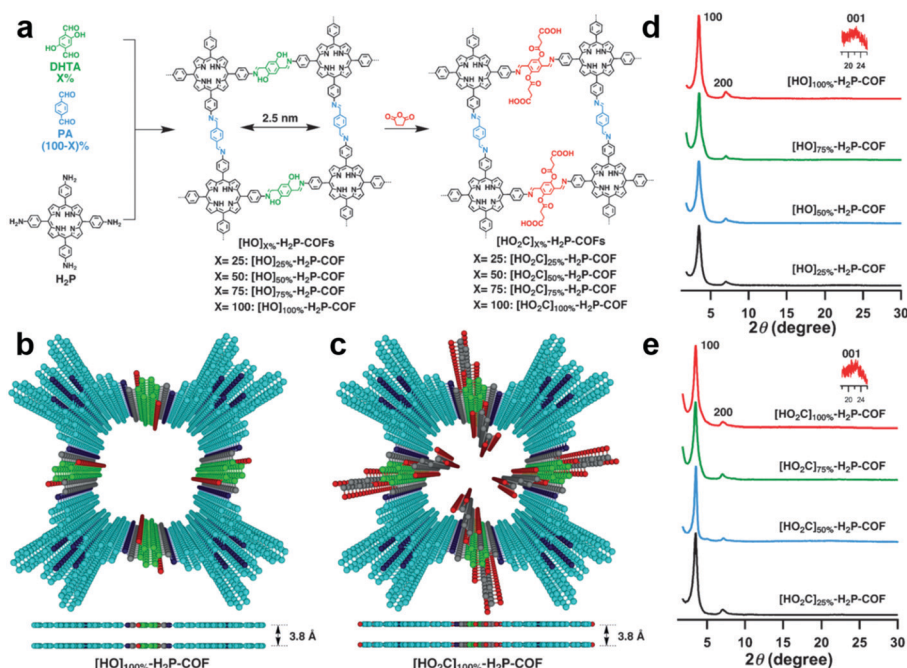
Fig. 7 (a) Synthesis of [HO 2 C] x% -H 2 P-COFs with channel walls functionalized with carboxylic acid groups through the ring opening reaction. Top views of (b) [HO] 100% -H 2 P-COF and (c) [HO 2 C] 100% -H 2 P-COF. XRD patterns of (d) [OH] x% -H 2 P-COFs and (e) [HO 2 C] x% -H 2 P-COFs. Reproduced with permission from ref. 106. Copyright 2017, Wiley-VCH.
