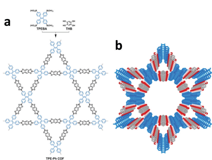
Fig. 8 (a) Synthesis of TPE-Ph COF from the condensation of TPEBA and THB. (b) Crystal structure of TPE-Ph COF with AA stacking mode. Fluorescence microscopy images of TPE-Ph COF samples synthesized in (c) 3 days (d) 30 days (the yellow insert depicts an enlarged view of the belts). (e) Comparative fluorescence quantum yields of TPE-Ph COF and the model compound dispersed in cyclohexane and toluene, as well as in the solid state. Adapted with permission from J. Am. Chem. Soc. , 2016, 138 , 5797–5800. Copyright 2016 American Chemical Society.
