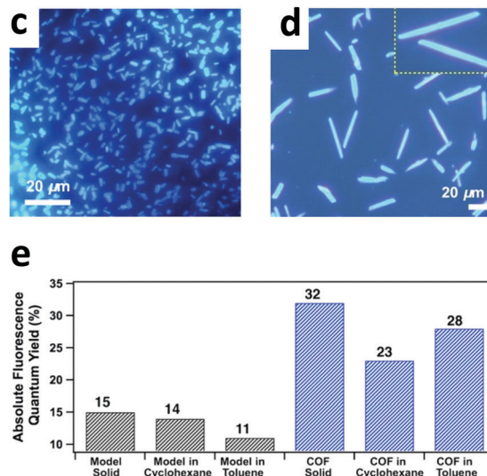
Fig. 8 (a) Synthesis of TPE-Ph COF from the condensation of TPEBA and THB. (b) Crystal structure of TPE-Ph COF with AA stacking mode. Fluorescence microscopy images of TPE-Ph COF samples synthesized in (c) 3 days (d) 30 days (the yellow insert depicts an enlarged view of the belts). (e) Comparative fluorescence quantum yields of TPE-Ph COF and the model compound dispersed in cyclohexane and toluene, as well as in the solid state. Adapted with permission from J. Am. Chem. Soc. , 2016, 138 , 5797–5800. Copyright 2016 American Chemical Society.
